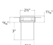
Section A-A FFED 65, FFDG 65, FFMN 65, FFAS 65
